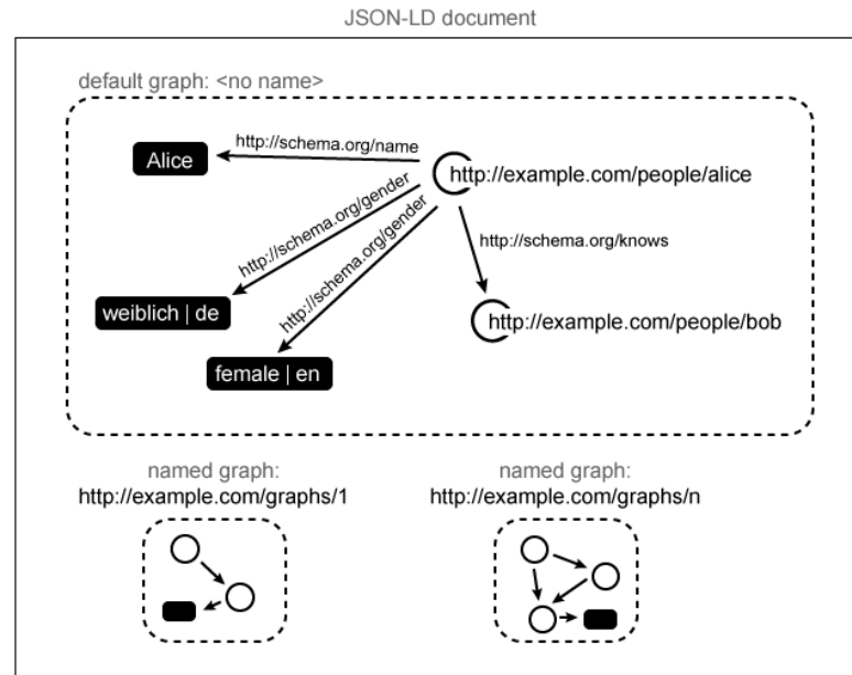
Figure 1: An illustration of the data model.
